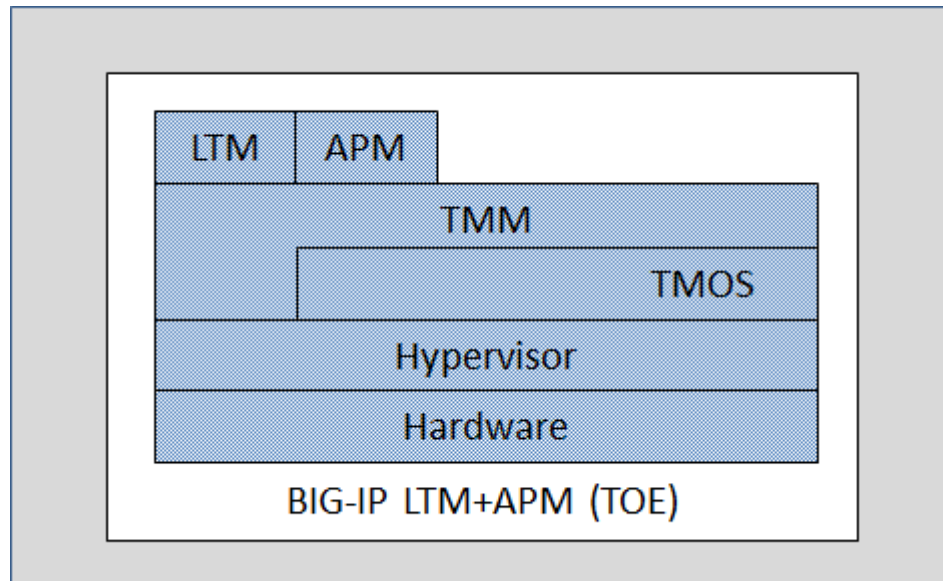
Figure 1: BIG-IP Subsystems
